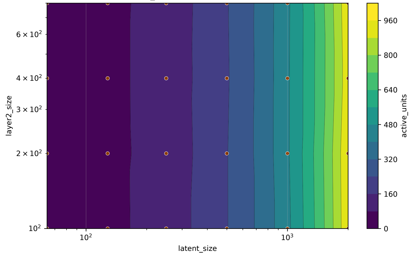
val/active_units (steps=start..2000, last)
