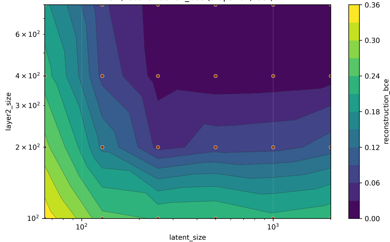
train/reconstruction_bce (steps=all, last)
