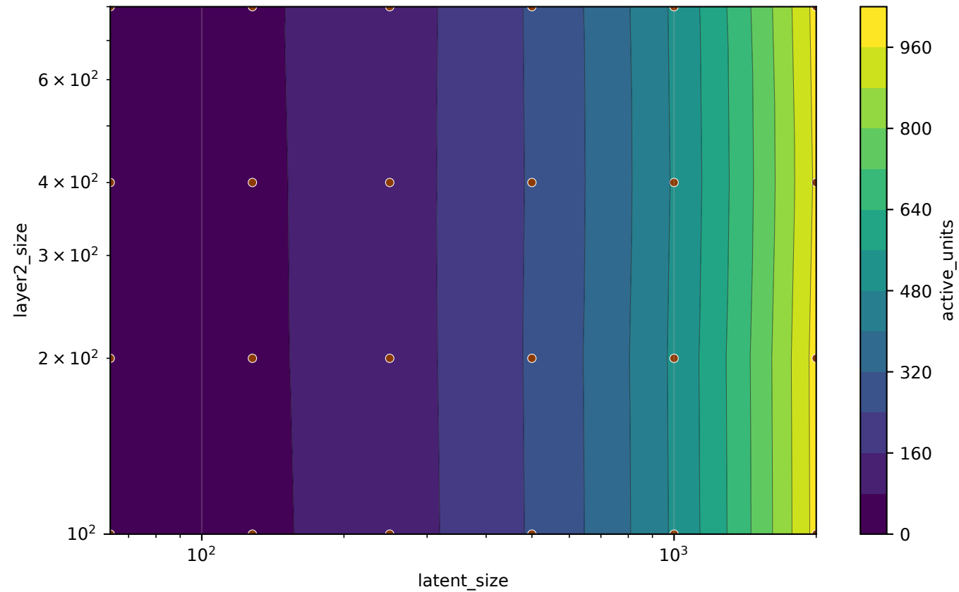
val/active_units (steps=all, last)
