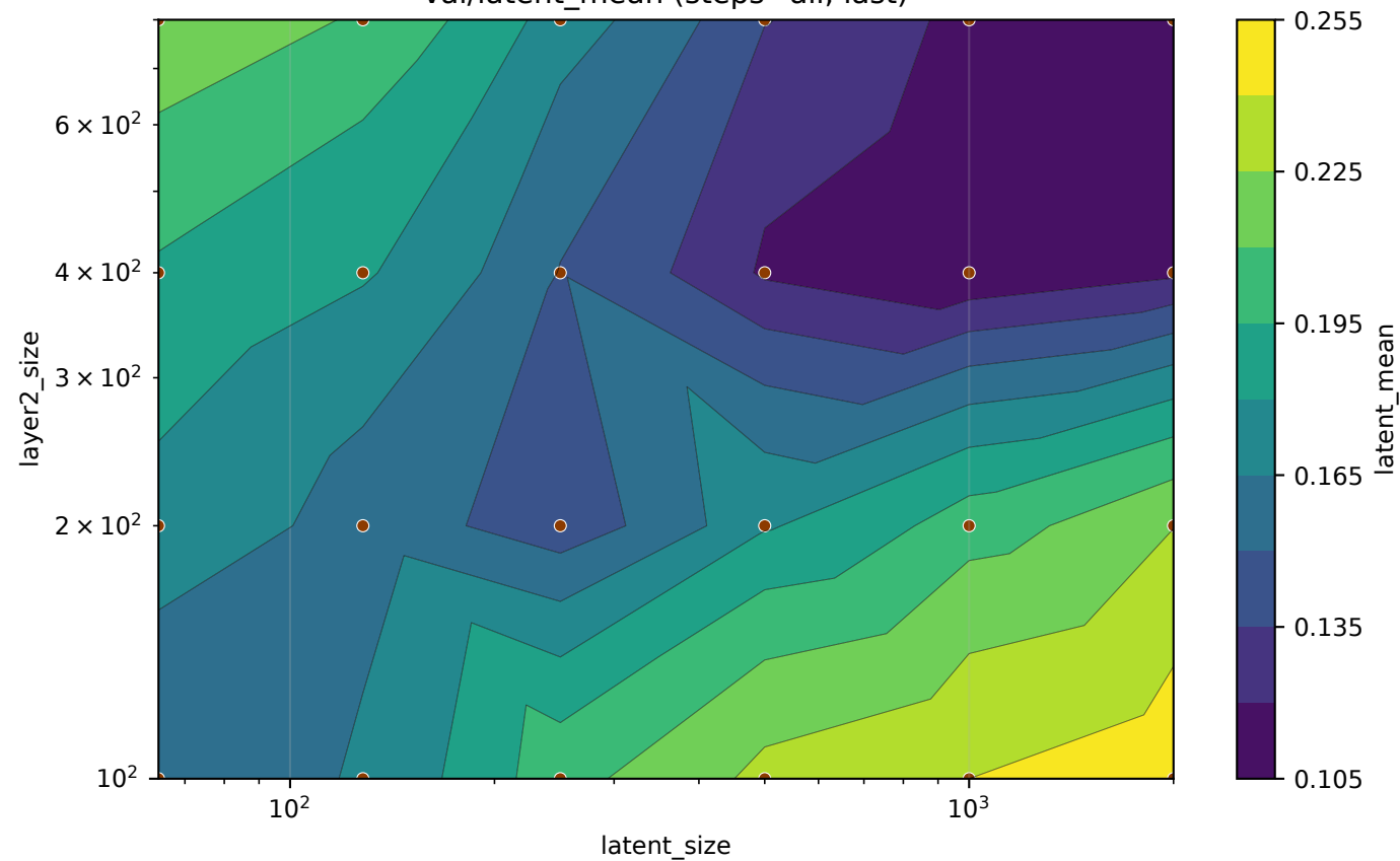
val/latent_mean (steps=all, last)
