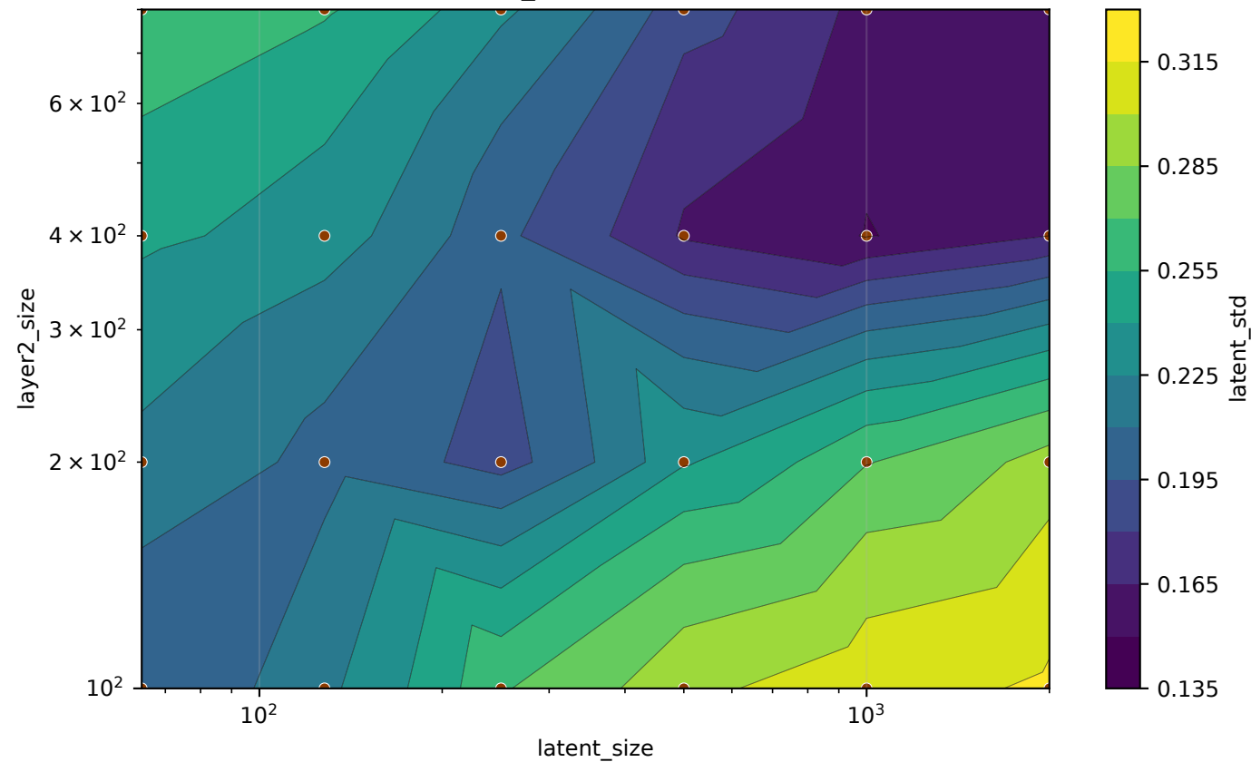
val/latent_std (steps=all, last)
