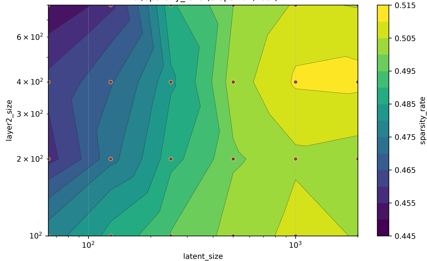
val/sparsity_rate (steps=all, last)
