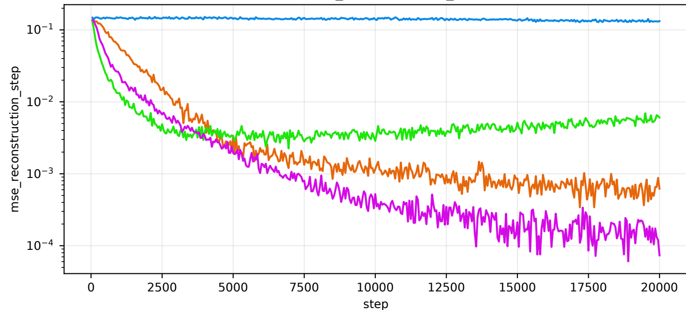
train/mse_reconstruction_step
