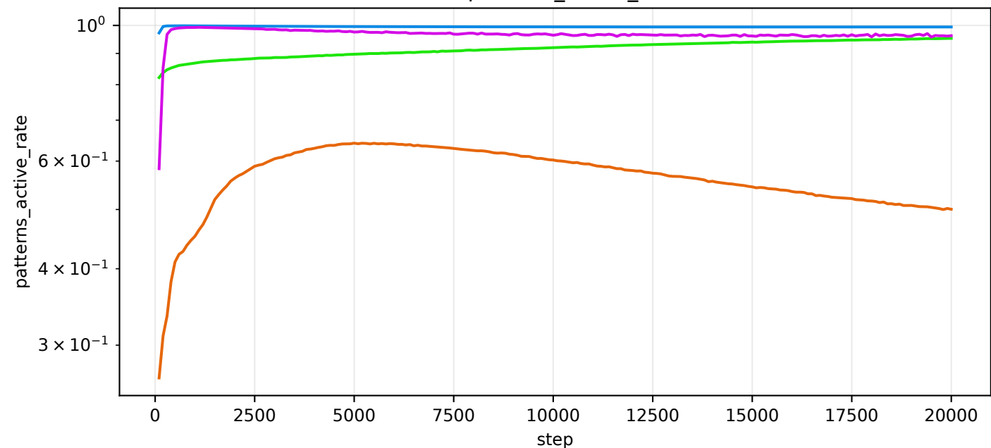
val/patterns_active_rate
