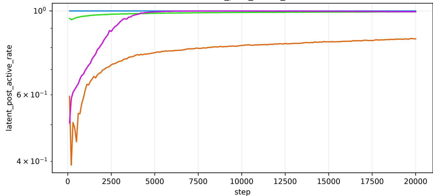
val/latent_post_active_rate
