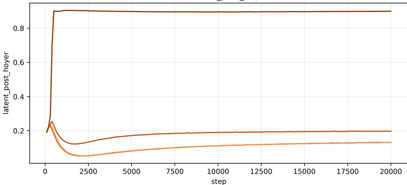
train/latent_post_hoyer
