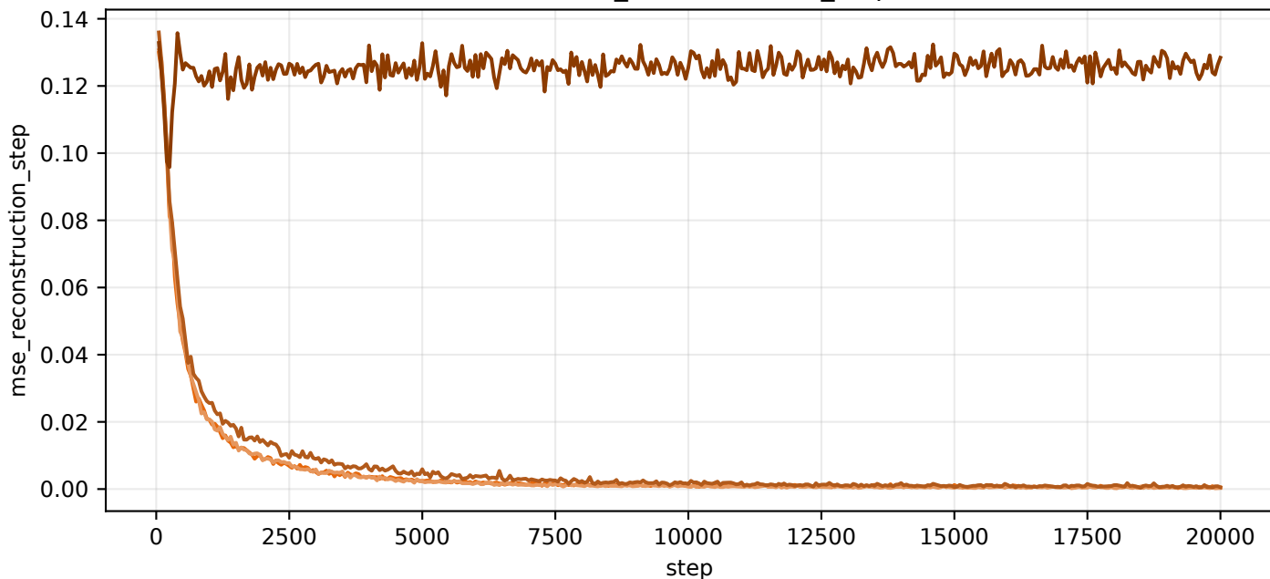
train/mse_reconstruction_step
