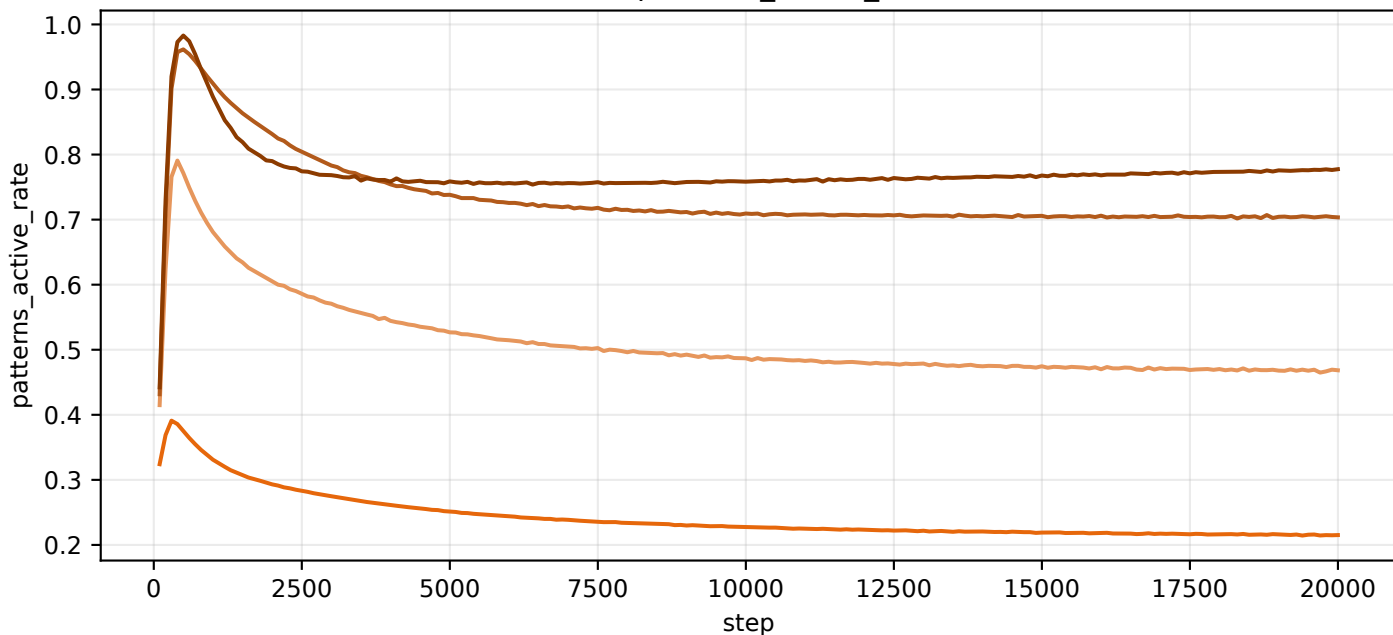
train/patterns_active_rate
