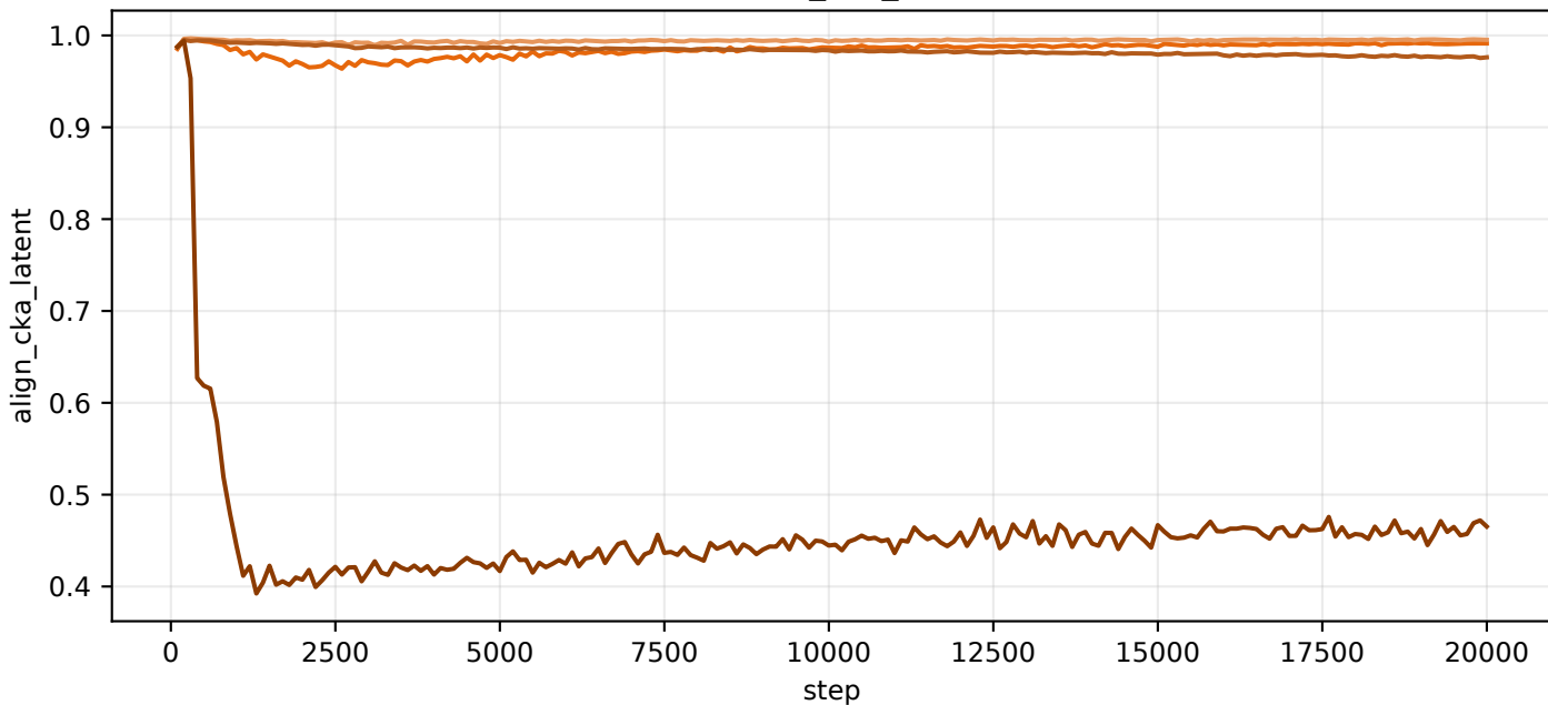
val/align_cka_latent
