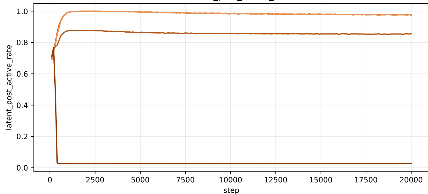
val/latent_post_active_rate
