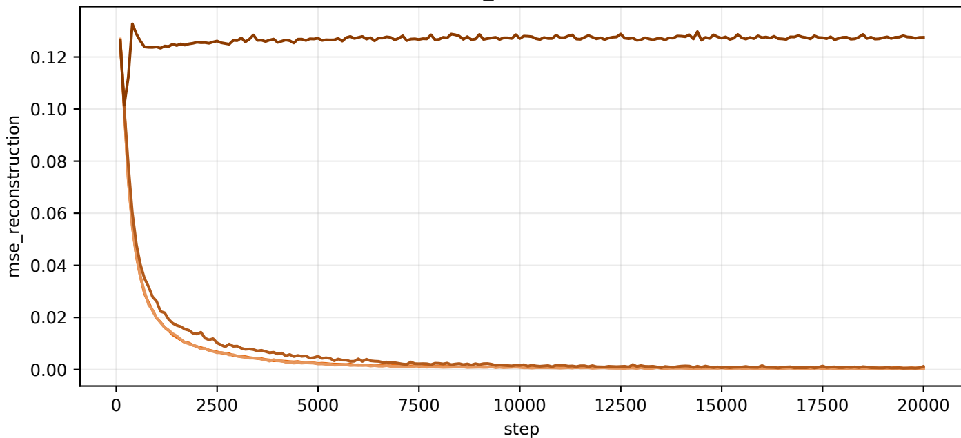
val/mse_reconstruction
