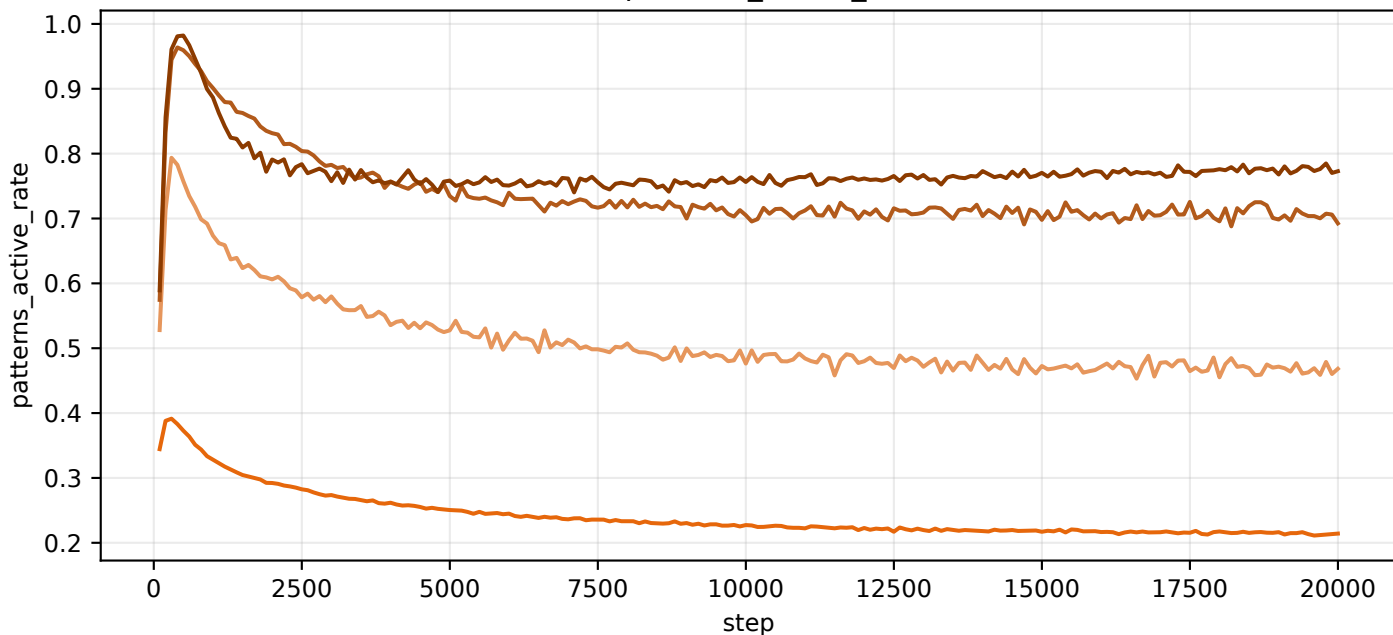
val/patterns_active_rate
