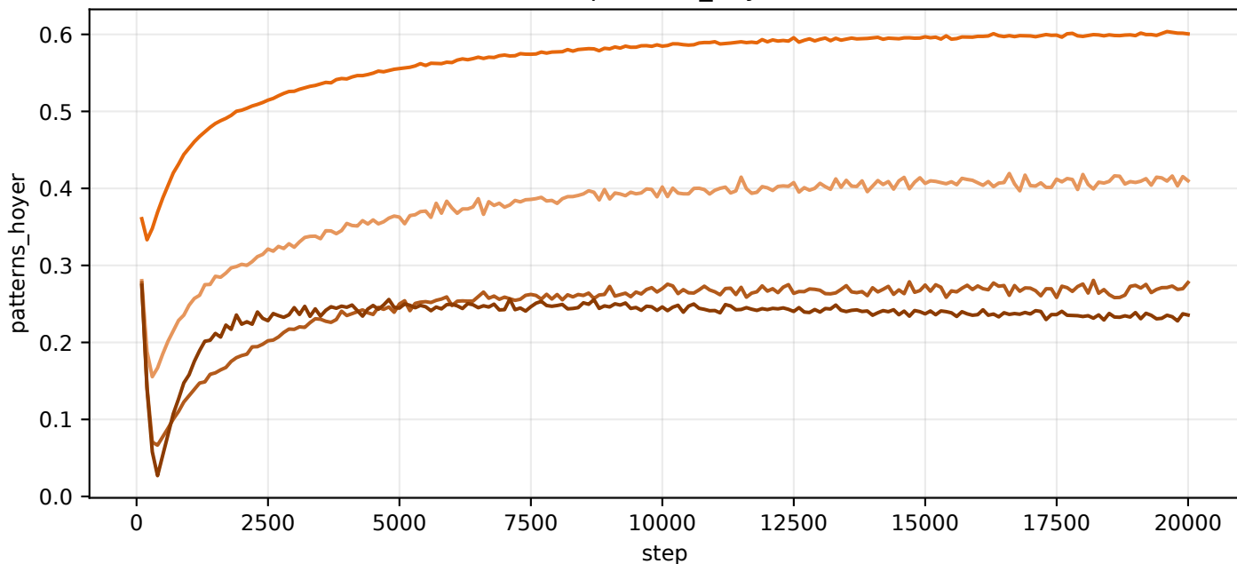
val/patterns_hoyer
