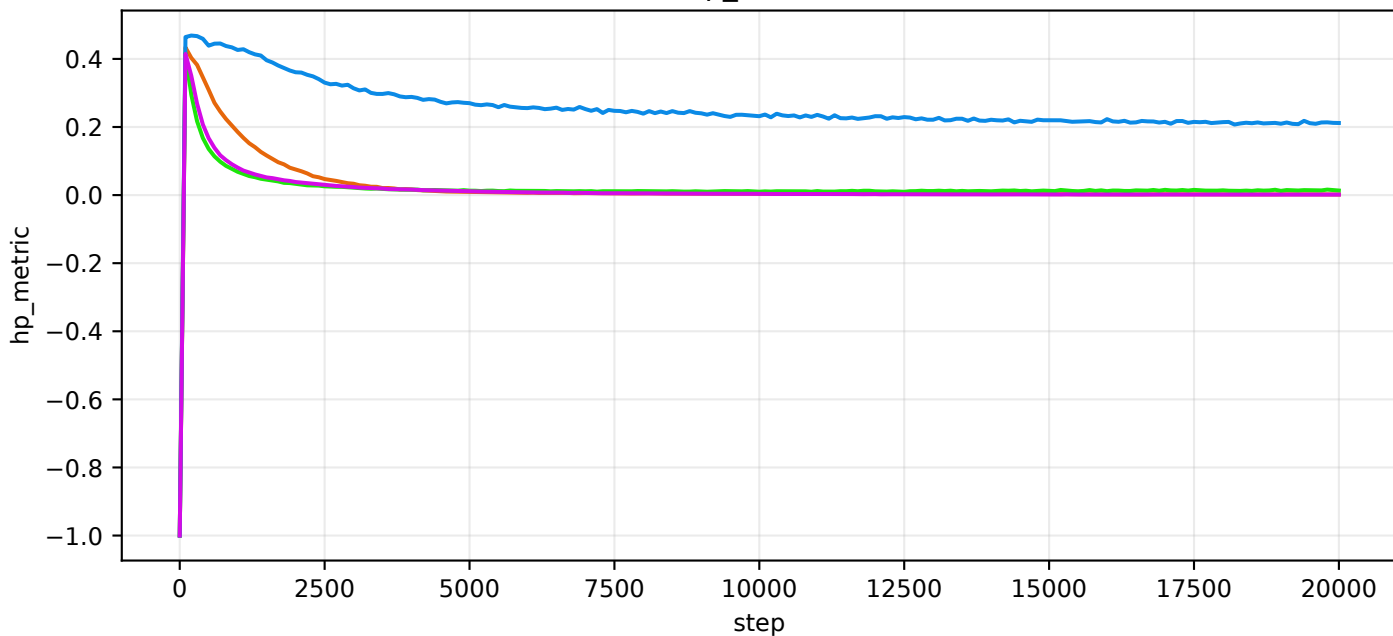
hp_metric
