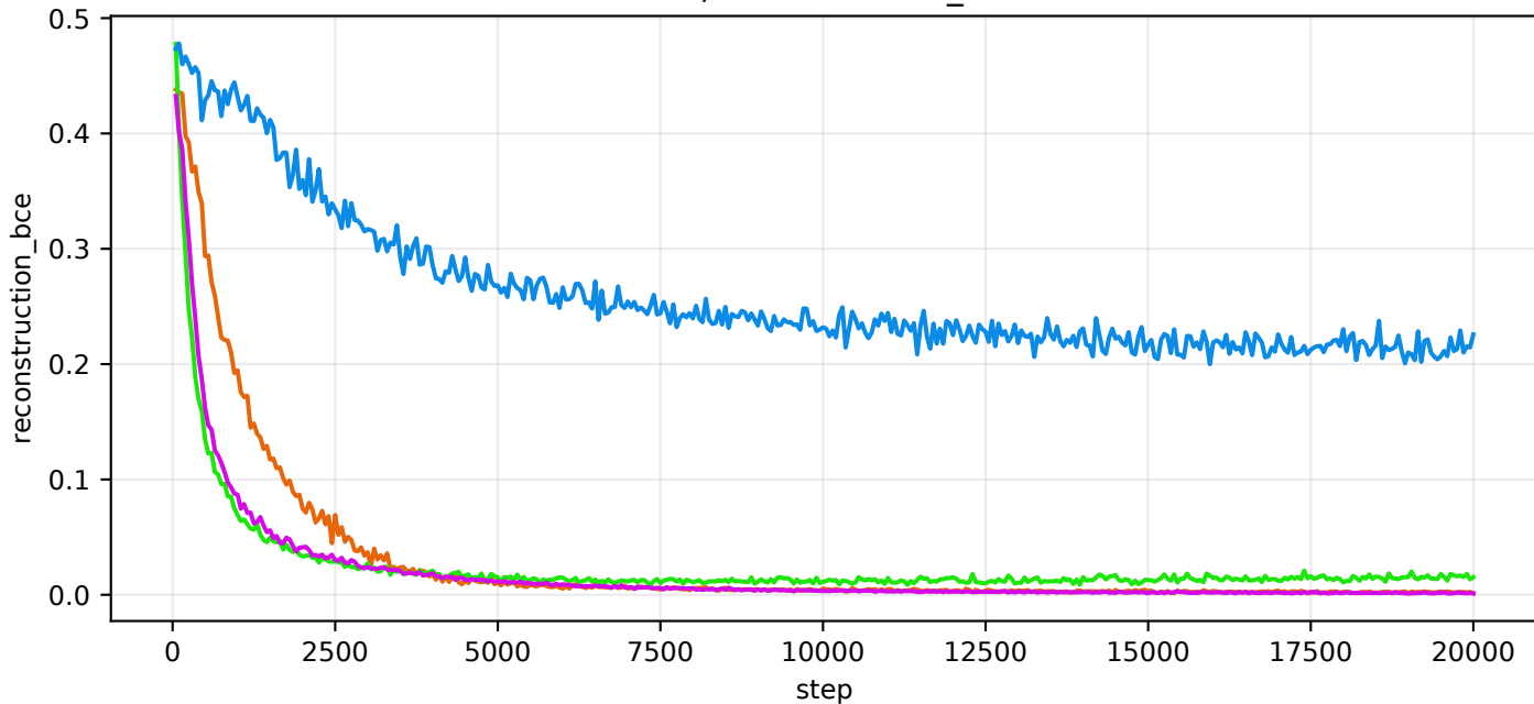
train/reconstruction_bce
