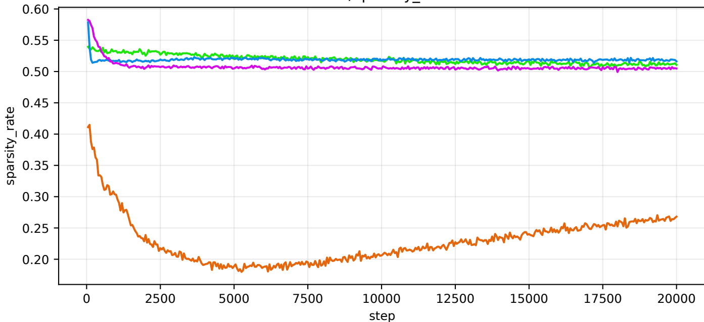
train/sparsity_rate
