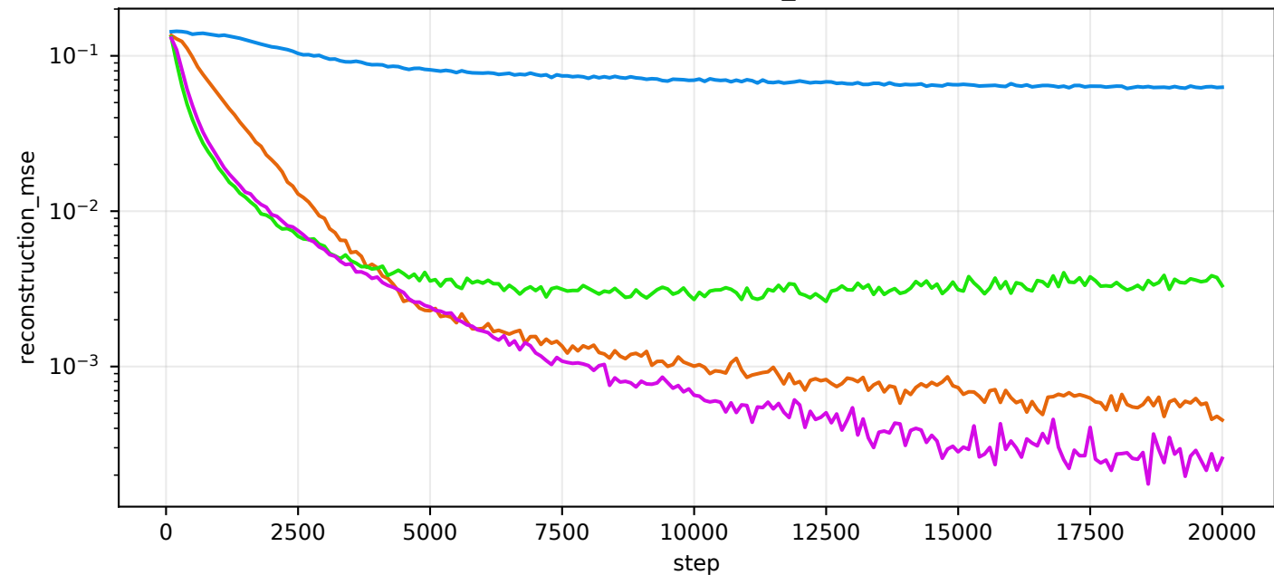
val/reconstruction_mse
