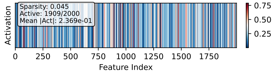
Activation Pattern
