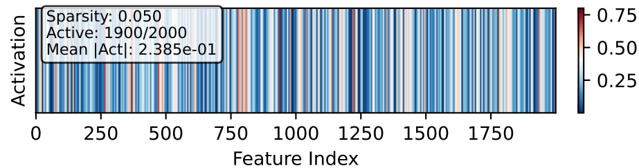
Activation Pattern
