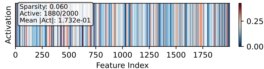
Activation Pattern
