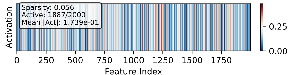
Activation Pattern
