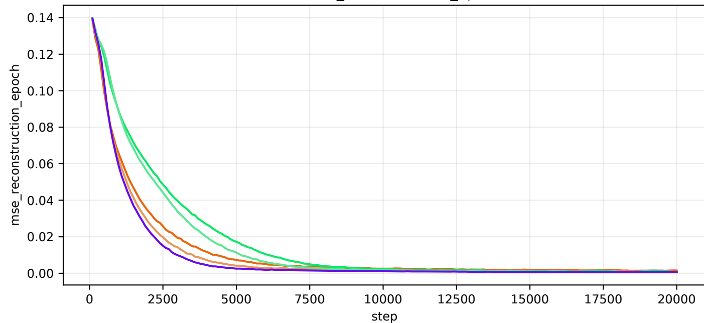
train/mse_reconstruction_epoch
