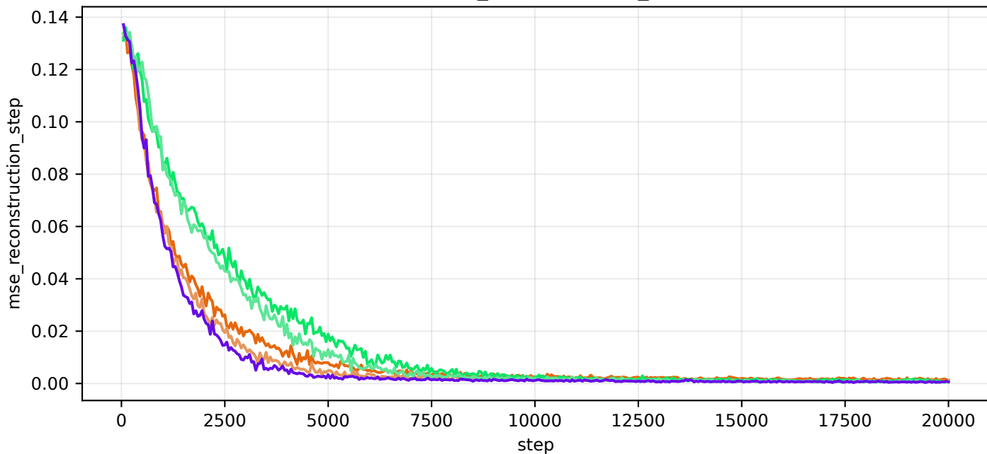
train/mse_reconstruction_step
