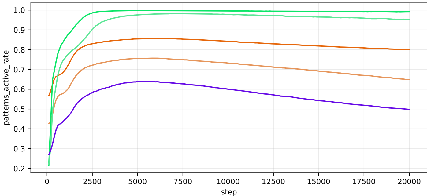
train/patterns_active_rate
