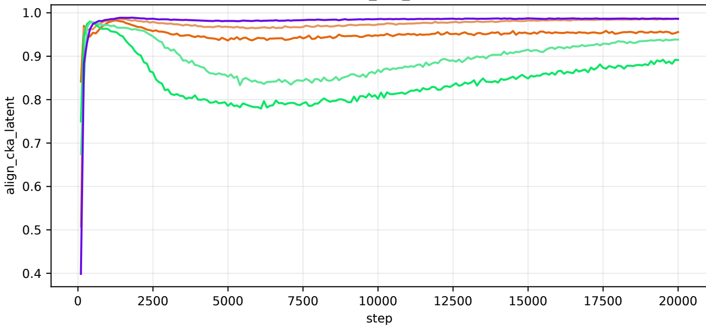
val/align_cka_latent
