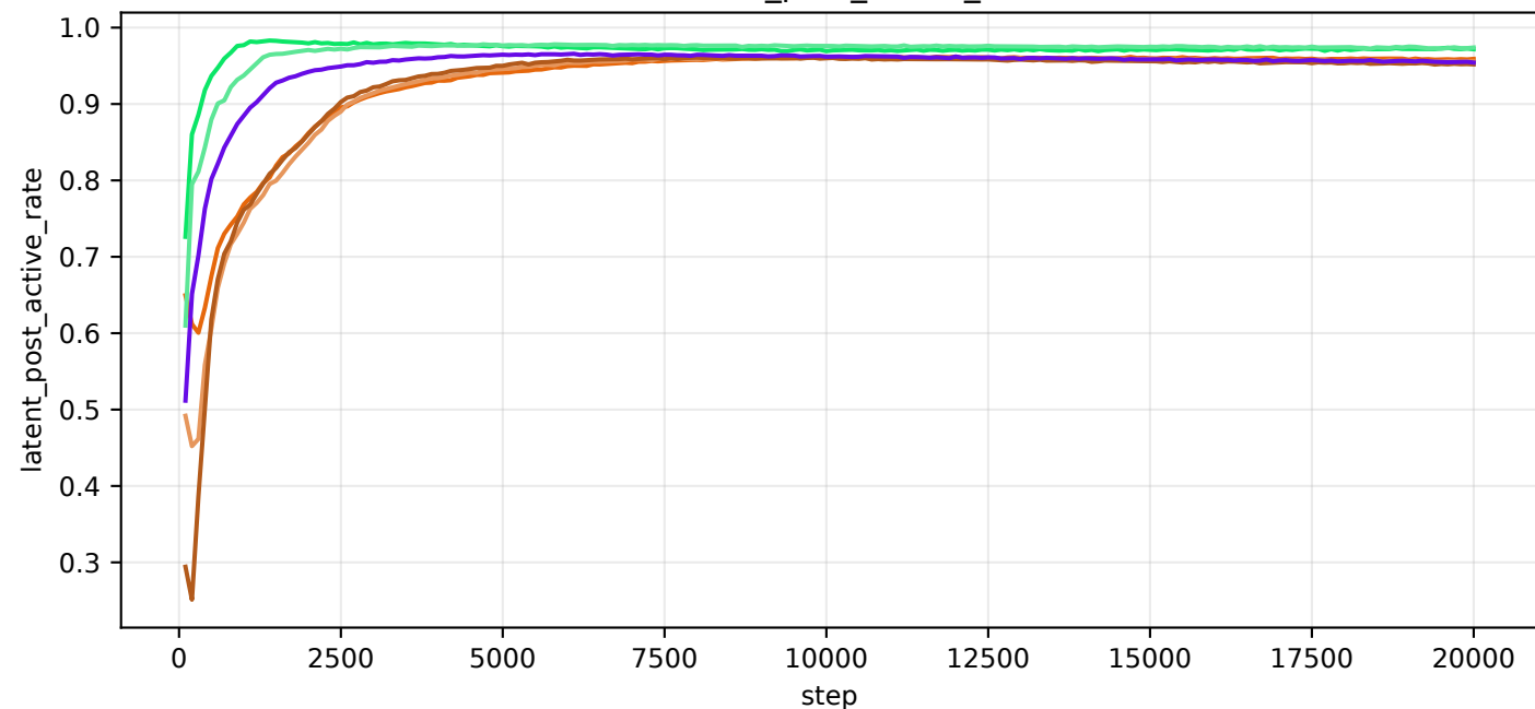
val/latent_post_active_rate
