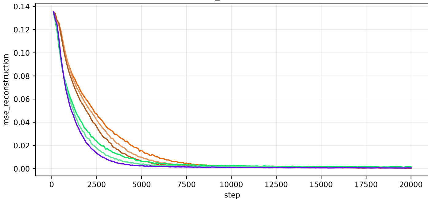
val/mse_reconstruction
