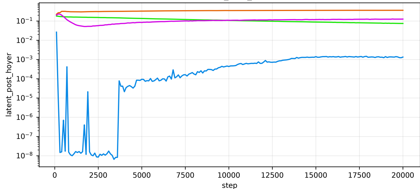
val/latent_post_hoyer
