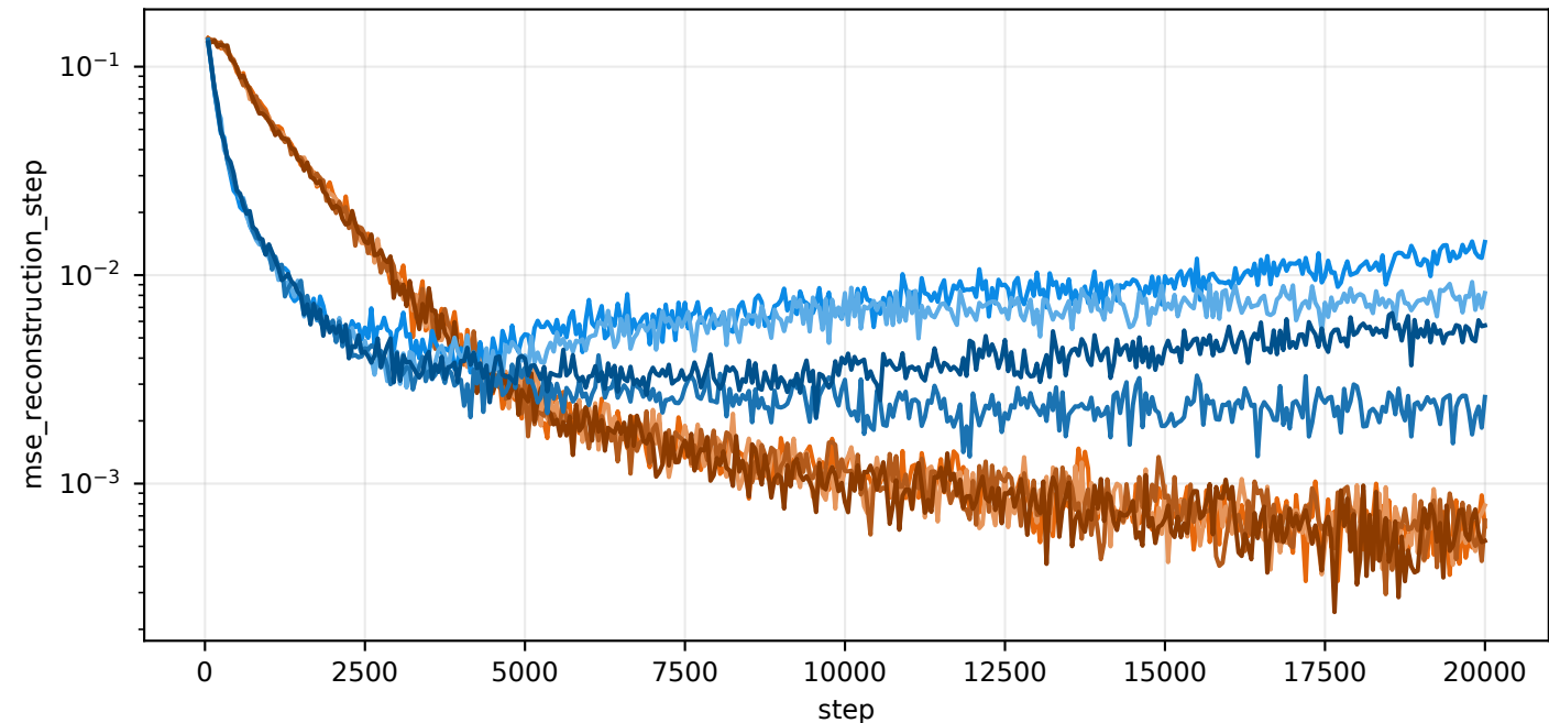
train/mse_reconstruction_step
