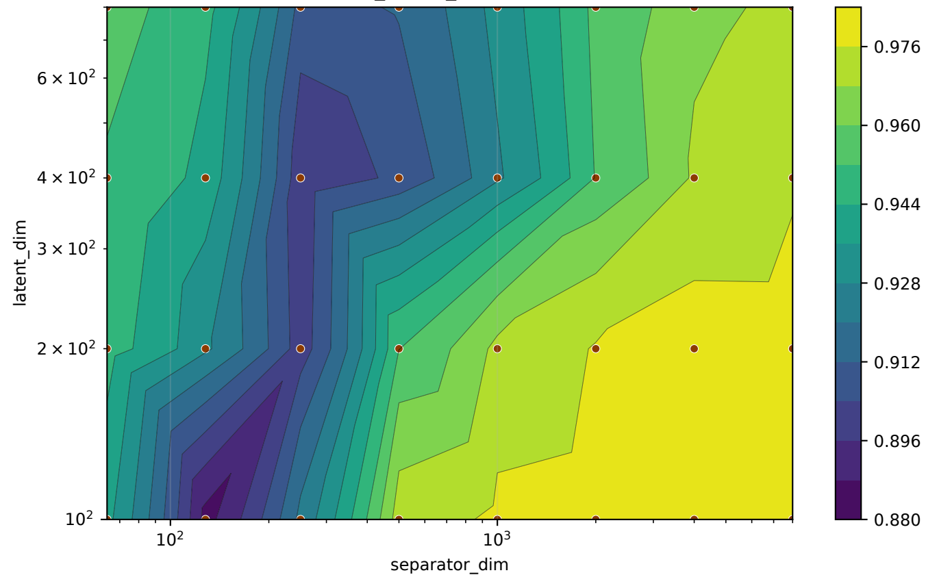
train/patterns_active_rate (steps=all, last)
