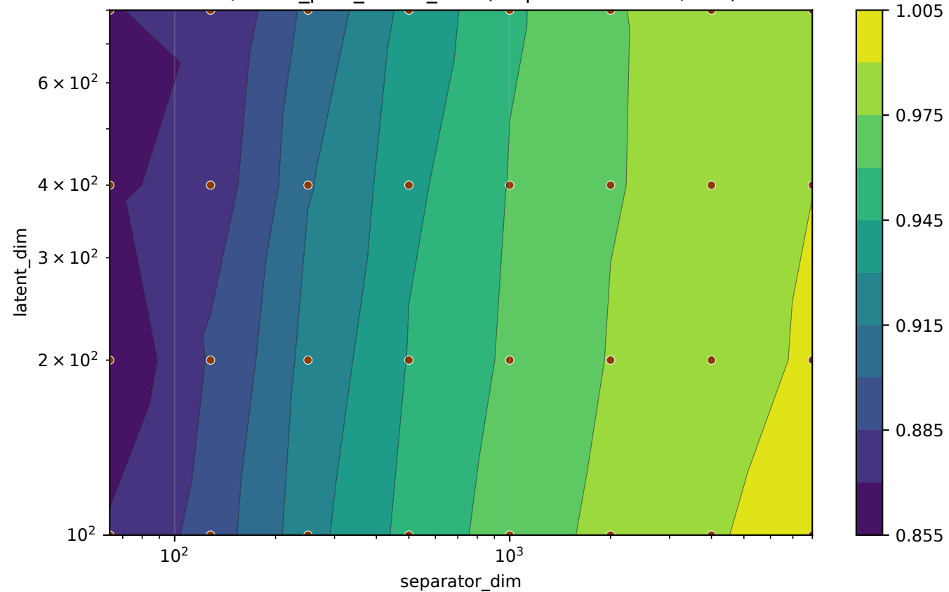
train/latent_post_active_rate (steps=start..2000, last)
