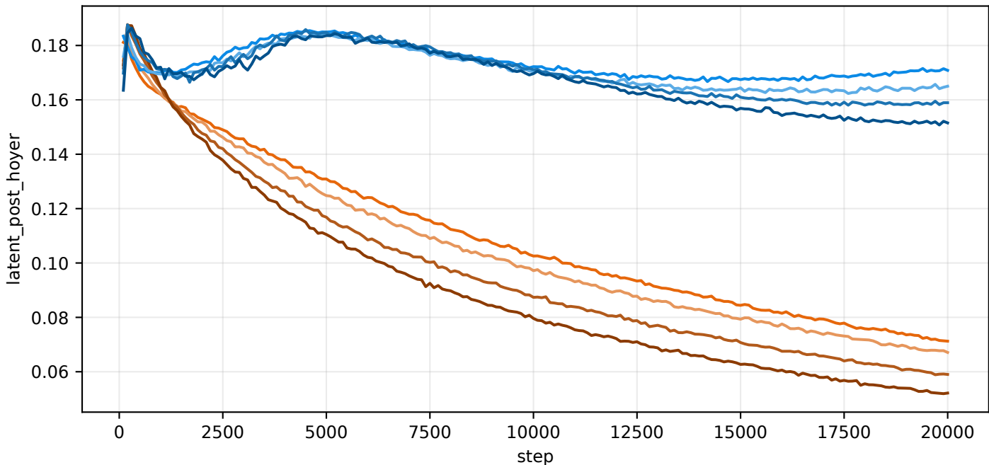
val/latent_post_hoyer
