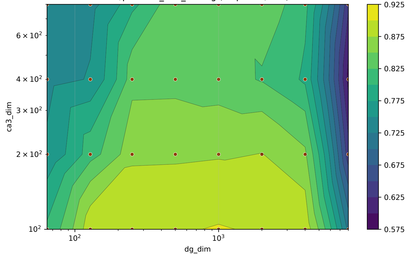
val/patterns_corr_offdiag (steps=all, last)
