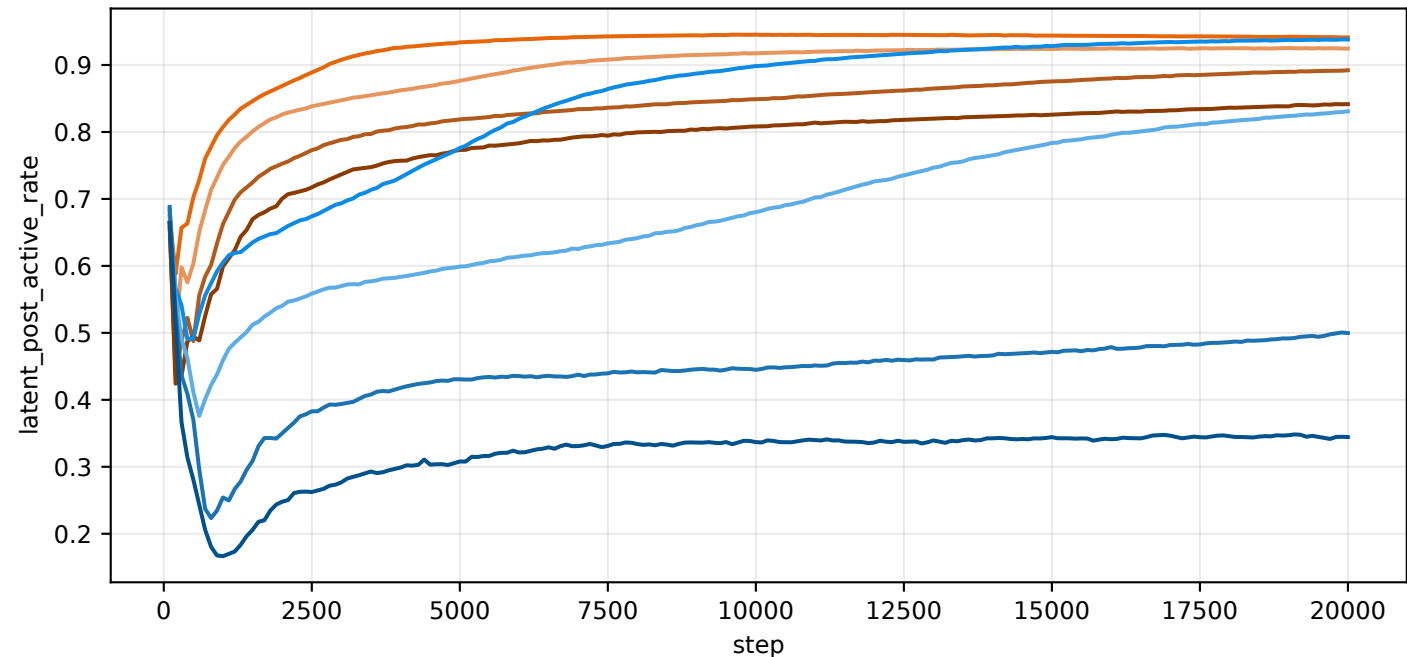
train/latent_post_active_rate
