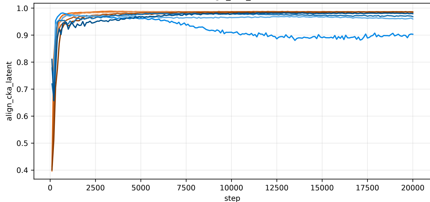
val/align_cka_latent
