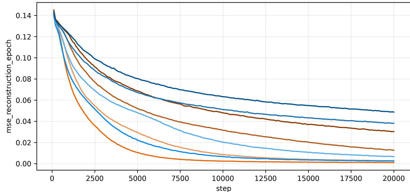
train/mse_reconstruction_epoch
