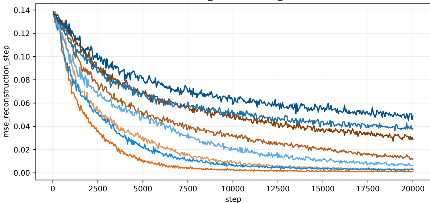
train/mse_reconstruction_step
