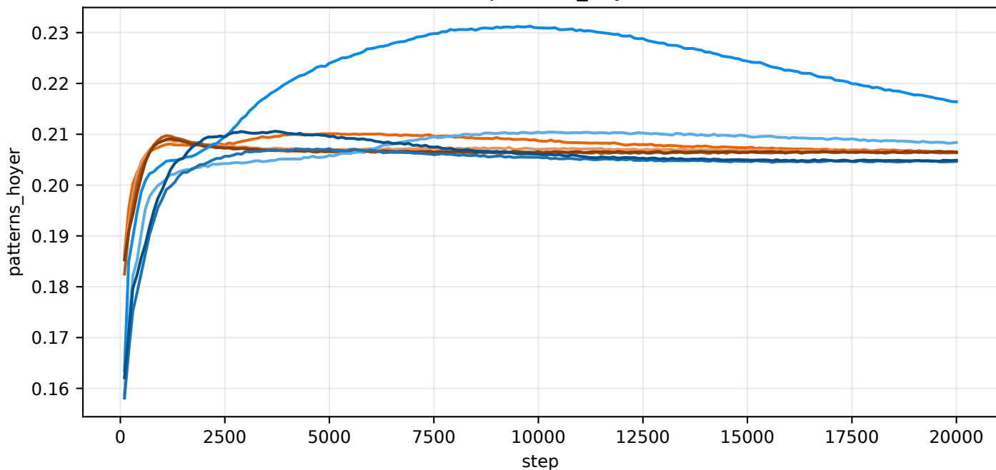
train/patterns_hoyer
