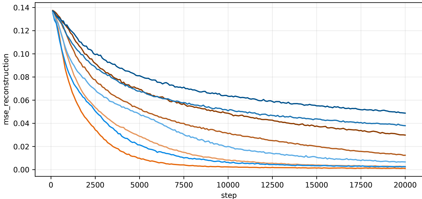
val/mse_reconstruction
