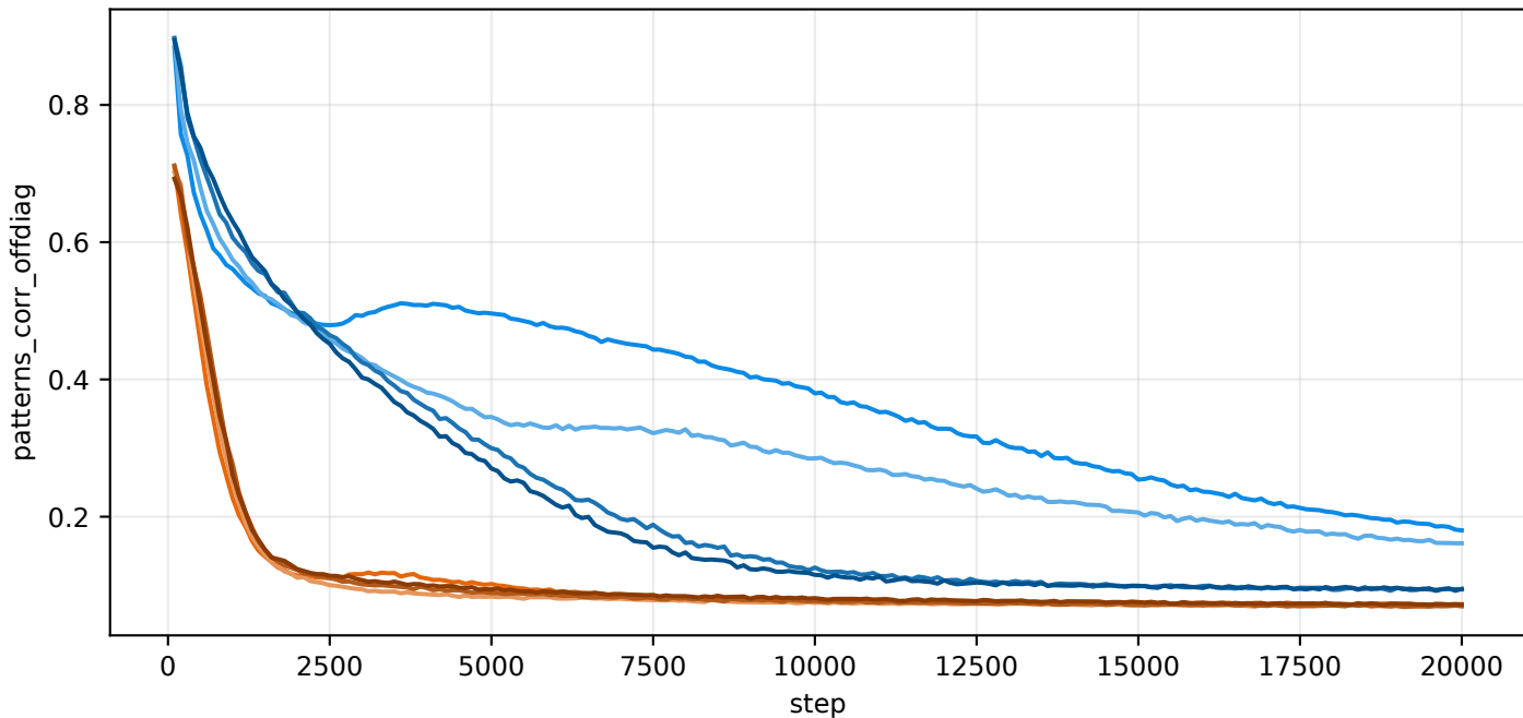
val/patterns_corr_offdiag
