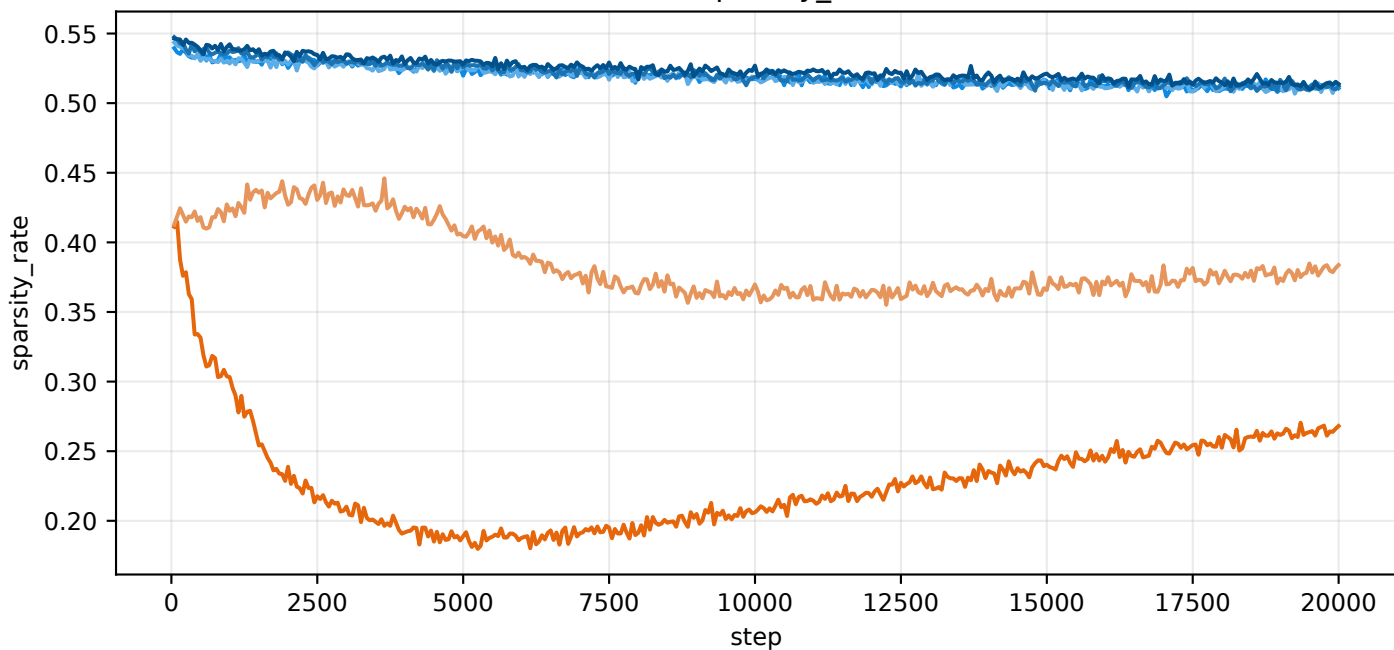
train/sparsity_rate
