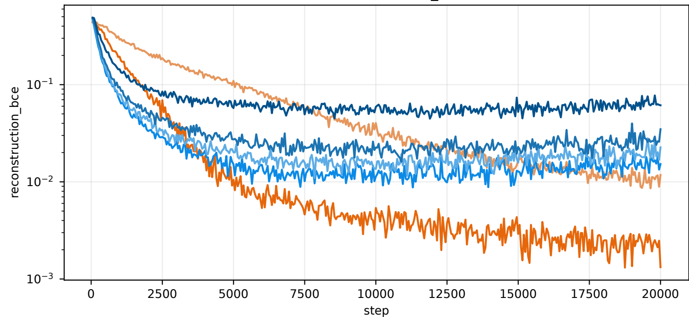
train/reconstruction_bce
