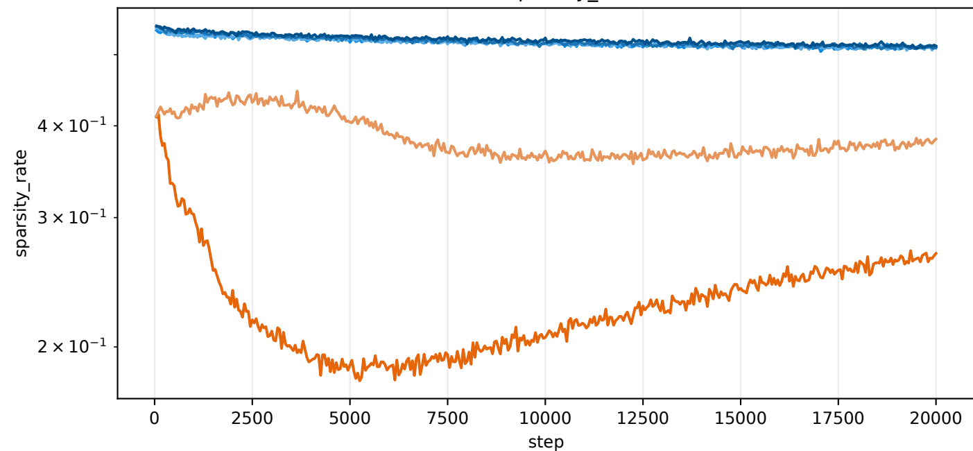
train/sparsity_rate
