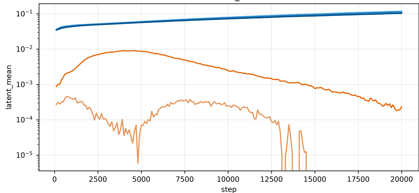
val/latent_mean
