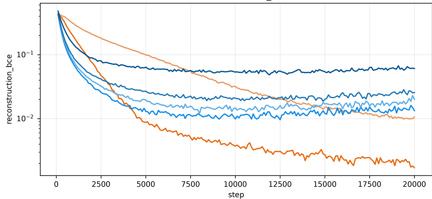
val/reconstruction_bce
