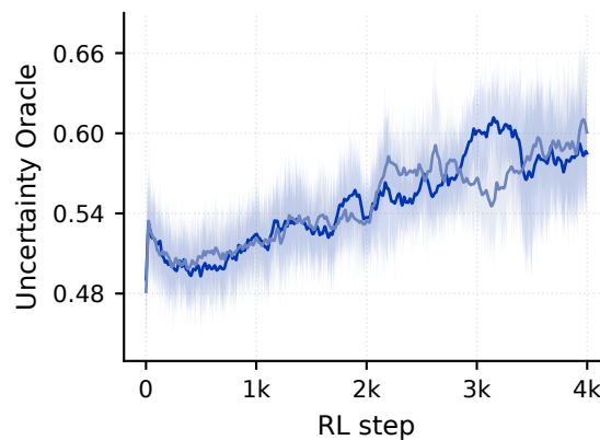
Uncertainty Oracle
