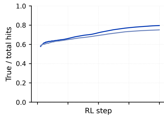
\Delta Predictor/Oracle
