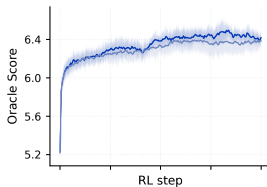
Uncertainty Oracle
