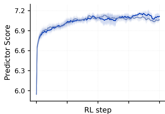
Uncertainty Predictor
