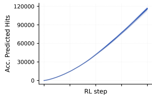
Predictor Score
