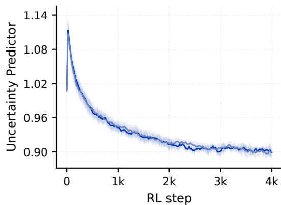
Uncertainty Predictor
