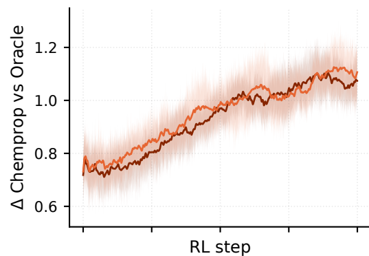
(i) Similarity EGFR
