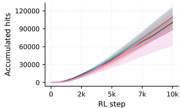
Accumulated Hits
